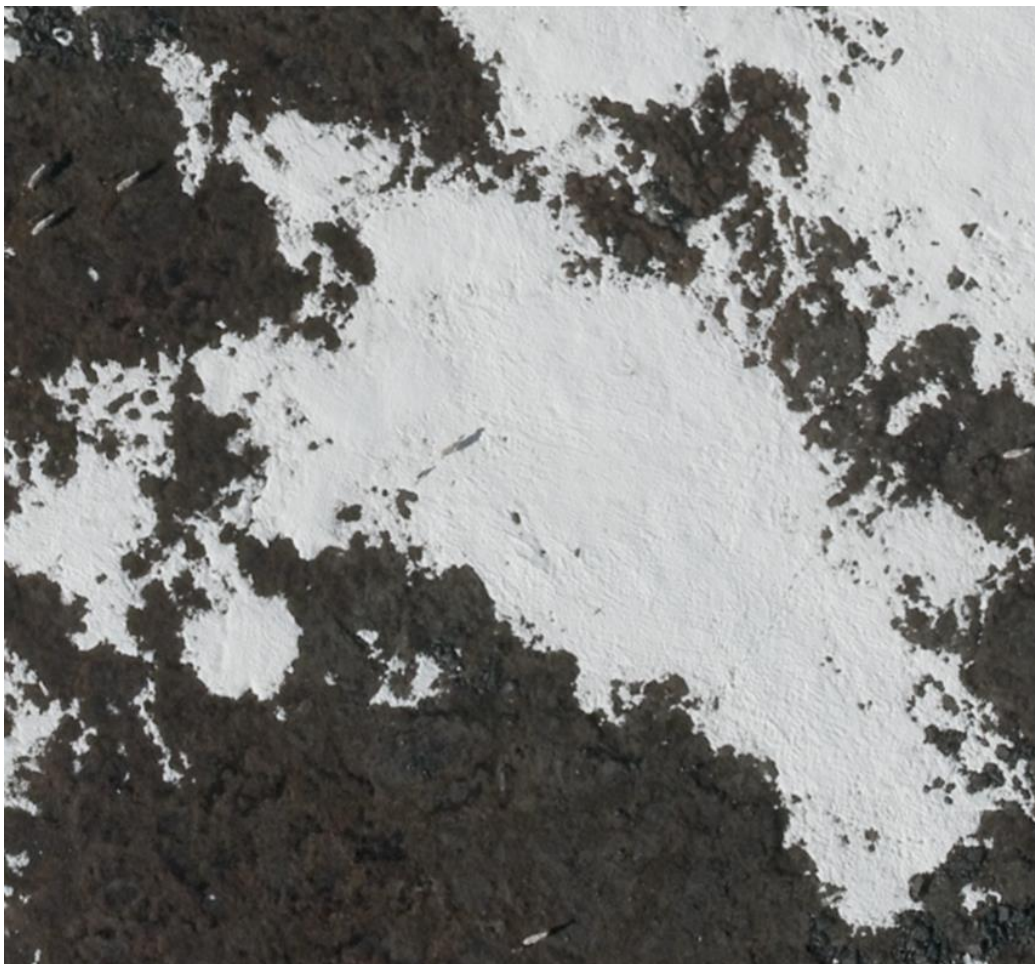
Figure 14: Close-up view of one zoomed-in portion of an aerial photo on Bluenose-East survey on June 8, 2018. Among others, three caribou are visible in the upper left corner, and a cow and calf can be seen walking (along with their shadows) across the snow-patch in the middle of the photo. Caribou in areas without snow are readily visible. There is also one caribou on the edge of the snow-patch at bottom right, which is less obvious.
