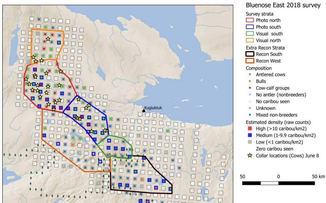
Figure 27: Bluenose-East June 2018 survey area with extra (post-hoc) reconnaissance-based strata at bottom in black and brown outlines.
