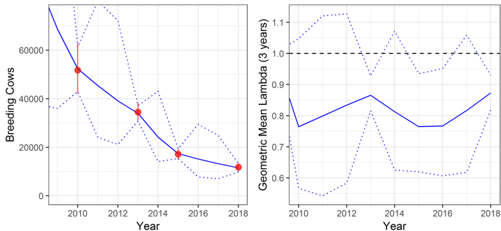
Figure 23: Estimates of breeding cows and \lambda (geometric mean of three previous years) in the Bluenose-East herd 2010-2018 from Bayesian state space model analysis.
