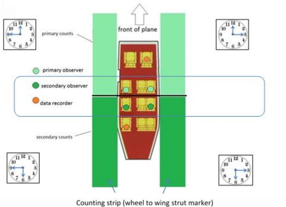
Figure 5: Observer and recorder positions for double observer methods on June 2018 caribou survey of Bluenose-East caribou. The secondary observer confirmed or called caribou not seen by the primary observer after the caribou have passed the main field of vision of the primary observer. Time on a clock can be used to reference relative locations of caribou groups (e.g. “caribou group at 1 o’clock”). The recorder was seated behind the two observers on the left side, with the pilot in the front seat. On the right side the recorder was seated at the front of the aircraft and was also responsible for navigating in partnership with the pilot.
