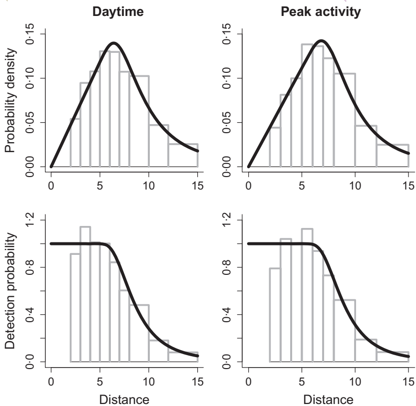
Fig. 4. Probability density functions of observed distances (top) and detection probability as a function of distance (bottom) from hazard-rate point transect models fit to data from Maxwell's duikers in Tai National Park, collected during the daytime (left) and during times of peak activity (right).
